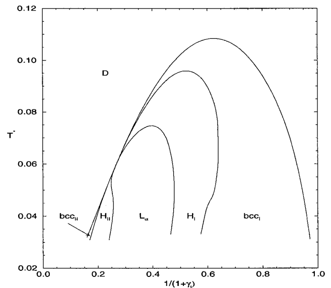
FIGURE 1 Phase diagram of the neutral lipid as a function of dimensionless temperature, T^* \equiv 1/2\chi N , and relative headgroup volume, 1/(1 + \gamma_i) . In addition to the disordered phase, D , there are normal and inverted body-centered cubic phases, bcc_I and bcc_{II} , normal and inverted hexagonal phases, H_I and H_{II} , and the lamellar phase L_\alpha .
