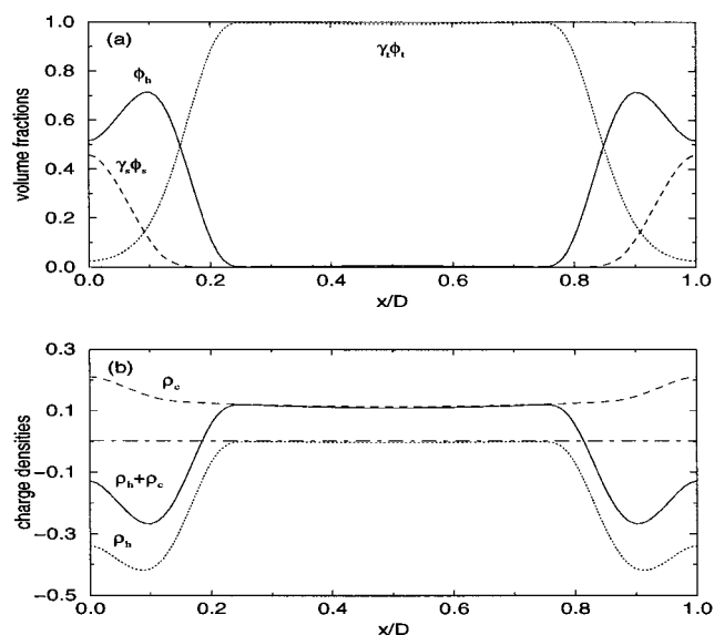
FIGURE 7 (a) Volume fraction distribution in the L_\alpha phase of the solvent, headgroups, and tails, in the system of Fig. 6 at a counter ion chemical potential of z_c = 0.1228 corresponding to the L_\alpha - H_{II} transition. The temperature is T^* = 0.04 , and the lattice parameter of the lamellar phase is D_L/R_g = 4.14 . (b) Charge densities arising from the headgroups, the counter ions, and the total charge density in the L_\alpha phase under the same conditions as in (a).
